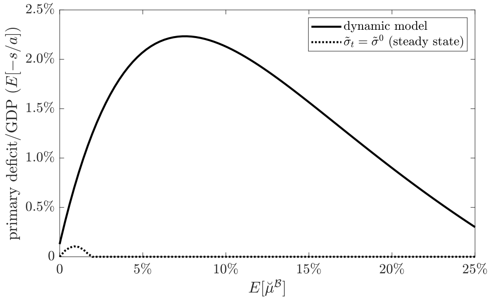
Figure 3: Debt Laffer curve for dynamic model and in steady state (constant \tilde{\sigma}_t ) when there is a bubble on government debt. \mathbb{E}[\tilde{\mu}^B] is varied by varying parameter \check{\mu}^{B,0} while keeping all other parameters as in Table 1.
