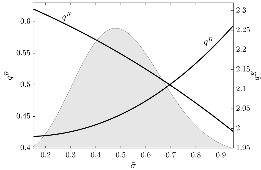
Figure 1: Equilibrium asset valuations q^B (left scale) and q^K (right scale) as a function of idiosyncratic risk \tilde{\sigma} . The gray shaded area in the background depicts the (rescaled) ergodic density of the state variable \tilde{\sigma} .
