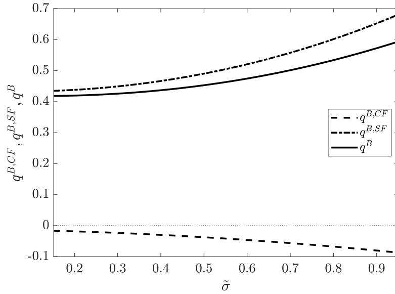
Figure 2: Decomposition of the value of government debt as a function of idiosyncratic risk \tilde{\sigma} . The dashed line shows the present value of primary surpluses ( q^{B,CF} ), the dashed-dotted line the present value of service flows ( q^{B,SF} ) and the solid line the total value of government debt ( q^B ), all normalized by the capital stock.
