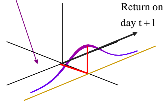
Conditional Distribution Net Return r_{t+1}
